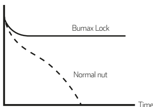
Fig 3. Residual stress
