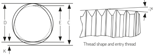
Taptite trilobular geometry
